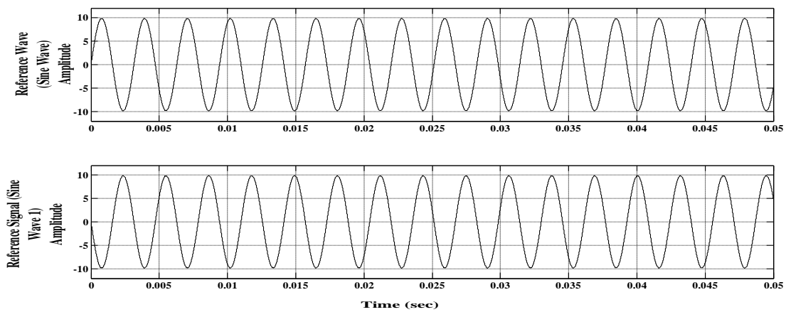
Fig.9. Waveform of Reference Wave for SPWM with unipolar voltage switching
