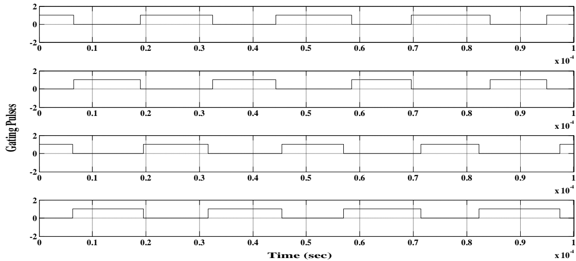
Fig.11. Switching Signal from Control Circuit for MOSFET T1, T2, T3, T4
