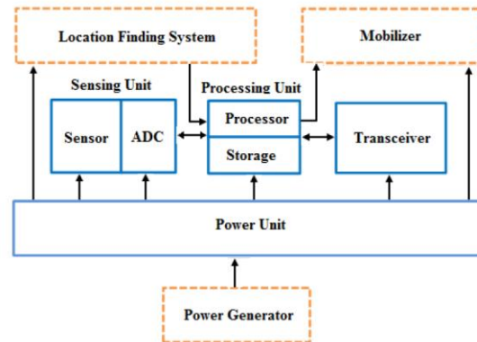
Fig 1 Components of typical sensor nodes
