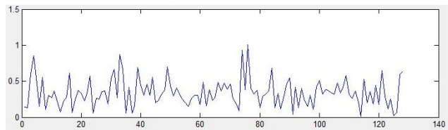
Figure 3: Transmitting Time Domain Signal for 64 carrier Nc-OFDM
