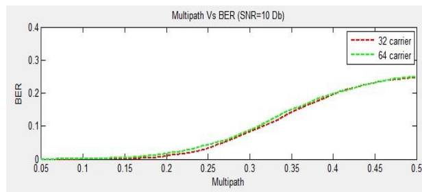
Figure 5: Multipath vs BER (SNR=10dB)
