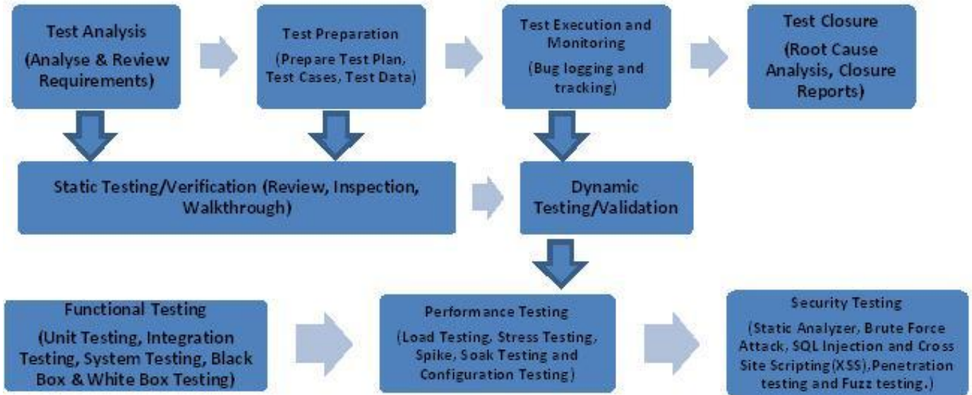
Fig. 6 Mapping of Software Test Phases and Testing Types
