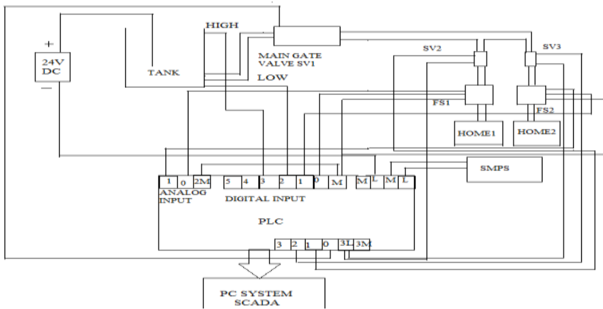
Fig no. 6 Wiring Diagram
