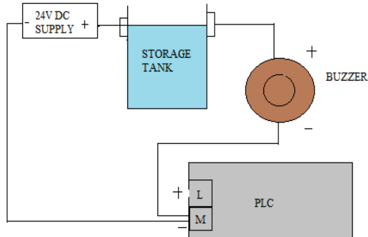
Fig.No.2 Level Measurement.
