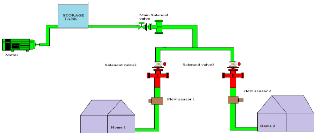
Fig.No.6 Pumping Section
