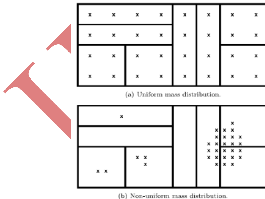
Fig. 2. Half space subdivisions of (a) uniform distribution (b) non uniform distribution
