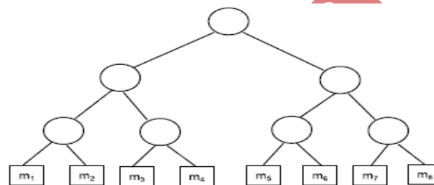
(a) HS-Tree.
